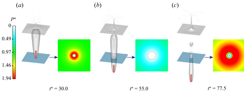
Figure 9. The cavity shape and the absolute pressure distributions in the cavity cross-section and the surrounding water at the measurement depth of z = -20D at several characteristic moments noted in figure 8. The water-entry velocity is v_0 = 100 \text{ m s}^{-1} ( Fr = 357.1 ), and the black line on the cross-section represents the cavity wall.
