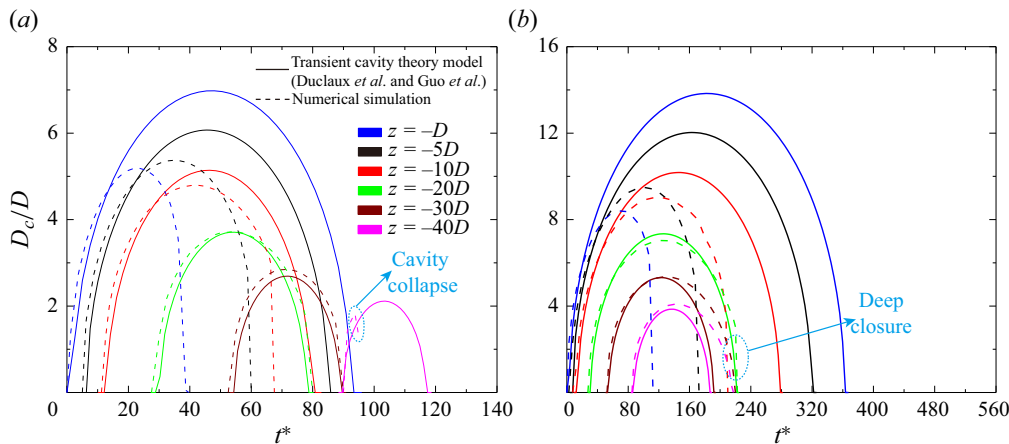
Figure 15. Comparisons between the theoretical predictions and numerical simulations of cavity diameter evolution at different depths. Panels show (a) v_0 = 100 \text{ m s}^{-1} , Fr = 357.1 ; (b) v_0 = 200 \text{ m s}^{-1} , Fr = 714.3 .
