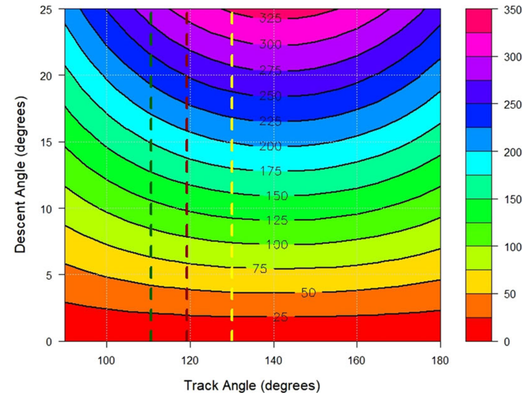
Figure 4. Variation of BFO error (Hz), compensated for horizontal motion, with track angle in degrees clockwise from north, and declination angle down from horizontal. The approximate aircraft to satellite direction is at 141.6° track angle (and elevation angle of 38.8°) where BFO changes are at a maximum across track angles for any given declination angle. At this track angle, BFO changes of over 325 Hz are possible for a declination angle of 25 degrees. Dashed lines refer to the different tracks in Figure 2: yellow is the ‘South track’; green is the ‘Adelaide track’; and red is the ‘PIC track’.
