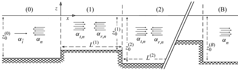
Figure 1. Definition sketch of multiple steps.
