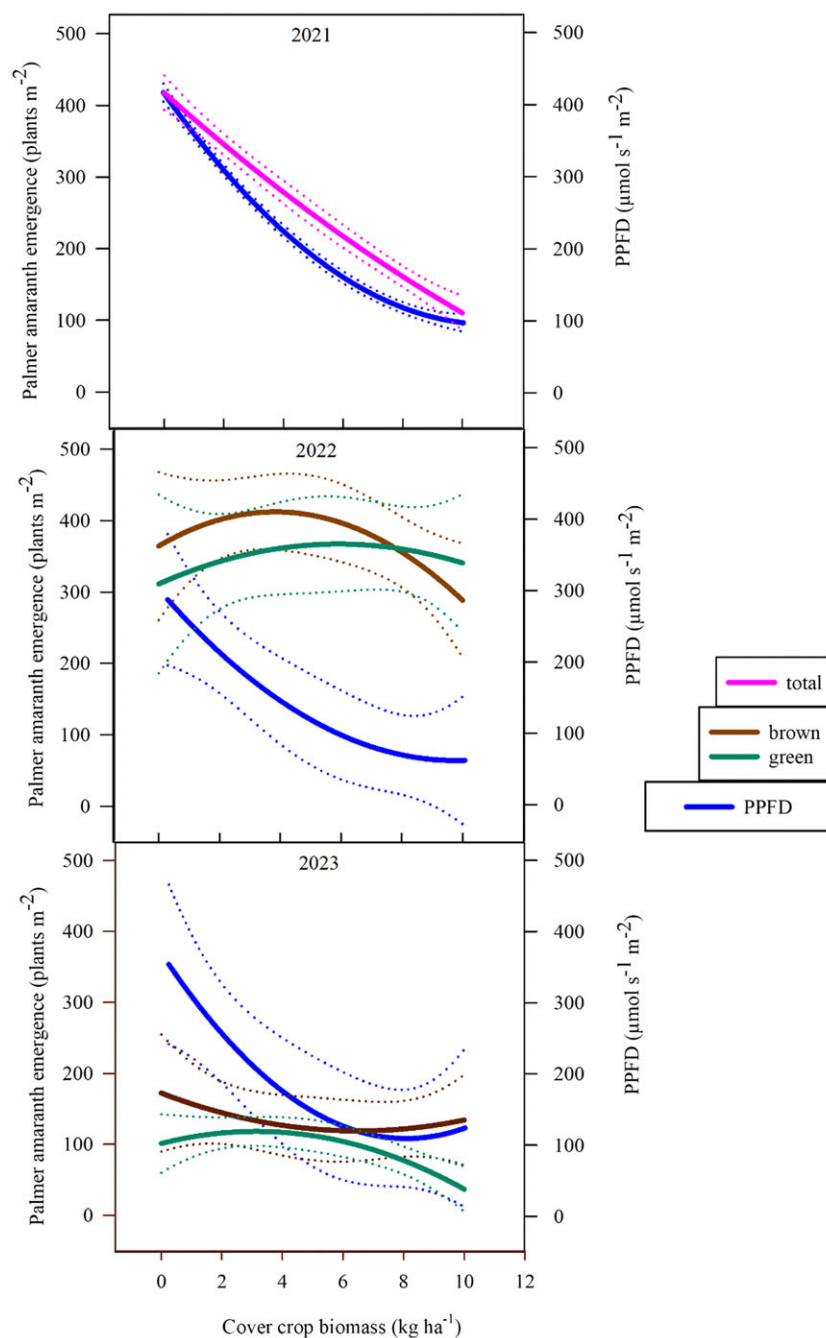
Figure 5. Greenhouse cumulative Palmer amaranth emergence for each experimental run from initiation to 4 wk after initiation (left axis) with average photosynthetic photon flux density (PPFD) (right axis) regressed across total cover crop (CC) biomass for experiments conducted between 2020 and 2023. The 2021 graph shows the main effect of CC biomass on total Palmer amaranth emergence, while the 2022 and 2023 graphs show the two-way interaction between termination timing (brown: CC terminated 2 wk prior to planting; green: CC terminated at the time of planting) and CC biomass. Dotted lines of the same color indicate 95% confidence intervals (see Table 2 for equation parameters).
