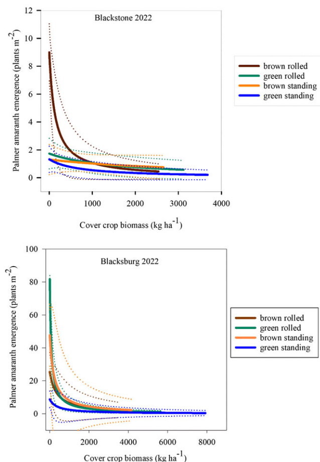
Figure 2. Regressions of significant three-way interactions at 6 wk after planting for Palmer amaranth emergence as a result of cover crop (CC) termination timing (brown: CC terminated 2 wk prior to planting; green: CC terminated at the time of planting), as well as rolled or standing, regressed across CC biomass for experiments conducted in Virginia between 2020 and 2023. Dotted lines of the same color indicate 95% confidence intervals (see Table 2 for equation parameters).
