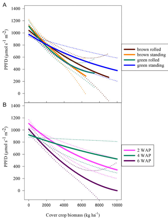
Figure 3. Photosynthetic photon flux density (PPFD) at soil level for trials conducted in Virginia between 2020 and 2023. A) PPFD at the soil surface level as a result of three-way interactions between termination timing (brown: cover crop [CC] terminated 2 wk prior to planting; green: CC terminated at the time of planting), rolled or standing, and the CC biomass gradient. B) PPFD as a result of two-way interactions between weeks after planting and CC biomass. Dotted lines of the same color indicate 95% confidence intervals (see Table 2 for equation parameters).
