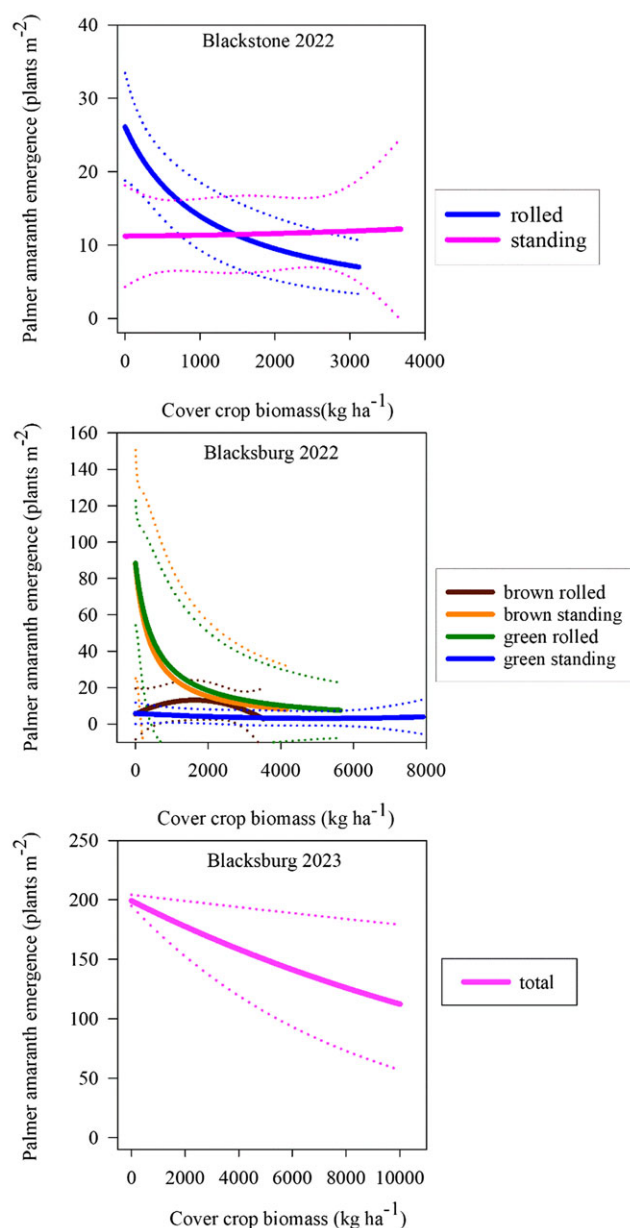
Figure 1. Palmer amaranth emergence for significant sites and interactions at 4 wk after planting (WAP) across cover crop (CC) biomass for experiments conducted in Virginia between 2020 and 2023. The top graph shows the relationship between Palmer amaranth emergence for the rolled and standing treatments across the CC biomass gradient. The middle graph shows the three-way interaction relationship for Palmer amaranth emergence as a result of termination timing (brown: CC terminated 2 wk prior to planting; green: CC terminated at the time of planting), rolled and standing, and the CC biomass gradient. The bottom graph shows total Palmer amaranth emergence across the main effect of CC biomass. Dotted lines of same color indicate 95% confidence intervals (see Table 2 for equation parameters).
