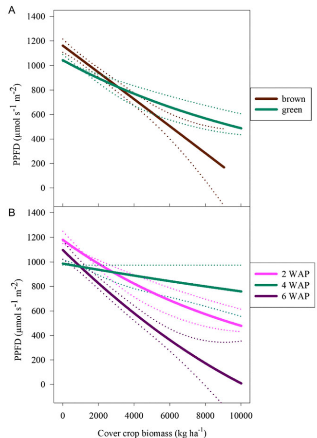
Figure 4. Photosynthetic photon flux density (PPFD) for all standing plots, including soil level, 15 cm, and 35 cm above the soil level for experiments conducted in Virginia between 2020 and 2023. A) Two-way interaction between termination timing (brown: cover crop [CC] terminated 2 wk prior to planting; green: CC terminated at the time of planting) and CC biomass. B) Two-way interaction between weeks after planting and CC biomass. Dotted lines of the same color indicate 95% confidence intervals (see Table 2 for equation parameters).
