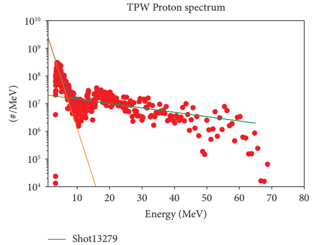
FIGURE 6: TPW data shot 13279, intensity 1.8 \times 10^{21} \text{ W/cm}^2 , 108 J in 144 fs, 50% energy focal radius of 4.1 \mu and strehl of 0.7.
