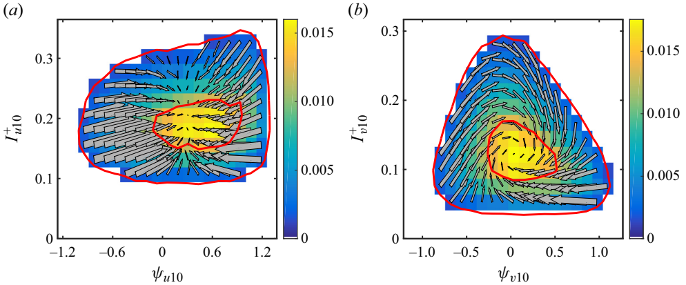
Figure 1. Probability distribution and flux vectors for two pairs of projection variables. The arrows link the centre of each partition cell with the mean location of the flow after a time iteration. The red contours enclose 0.3 and 0.95 of the probability mass. (a) A typical disorganised variable pair (Case I). (b) The well-organised Orr burst described in the text (Case II). Here \Delta t^* = 0.075 ; 21 \times 20 cells; C950 (adapted from Jiménez 2023).
