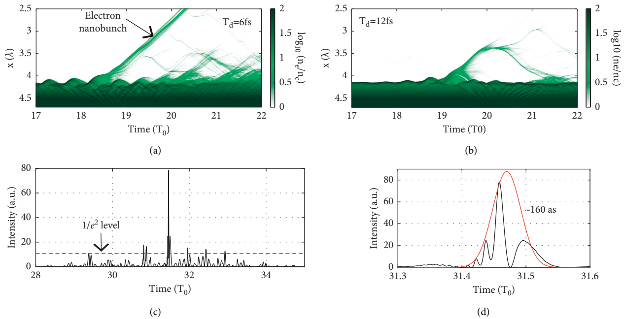
FIGURE 7: (a, b) The spatiotemporal evolution of electron density with delay T_d = 6 fs and 12 fs, respectively. (c) Obtained radiation pulse intensity by applying a spectral filter to select the 30th to 100th harmonic orders at T_d = 6 fs. (d) Zoomed view of a single pulse with envelope fitting (red). The other simulation parameters are a = 10 , \tau = 6 T_0 , L_s = 0.2 \lambda_L , n_e = 100 n_c , and normal incidence.
