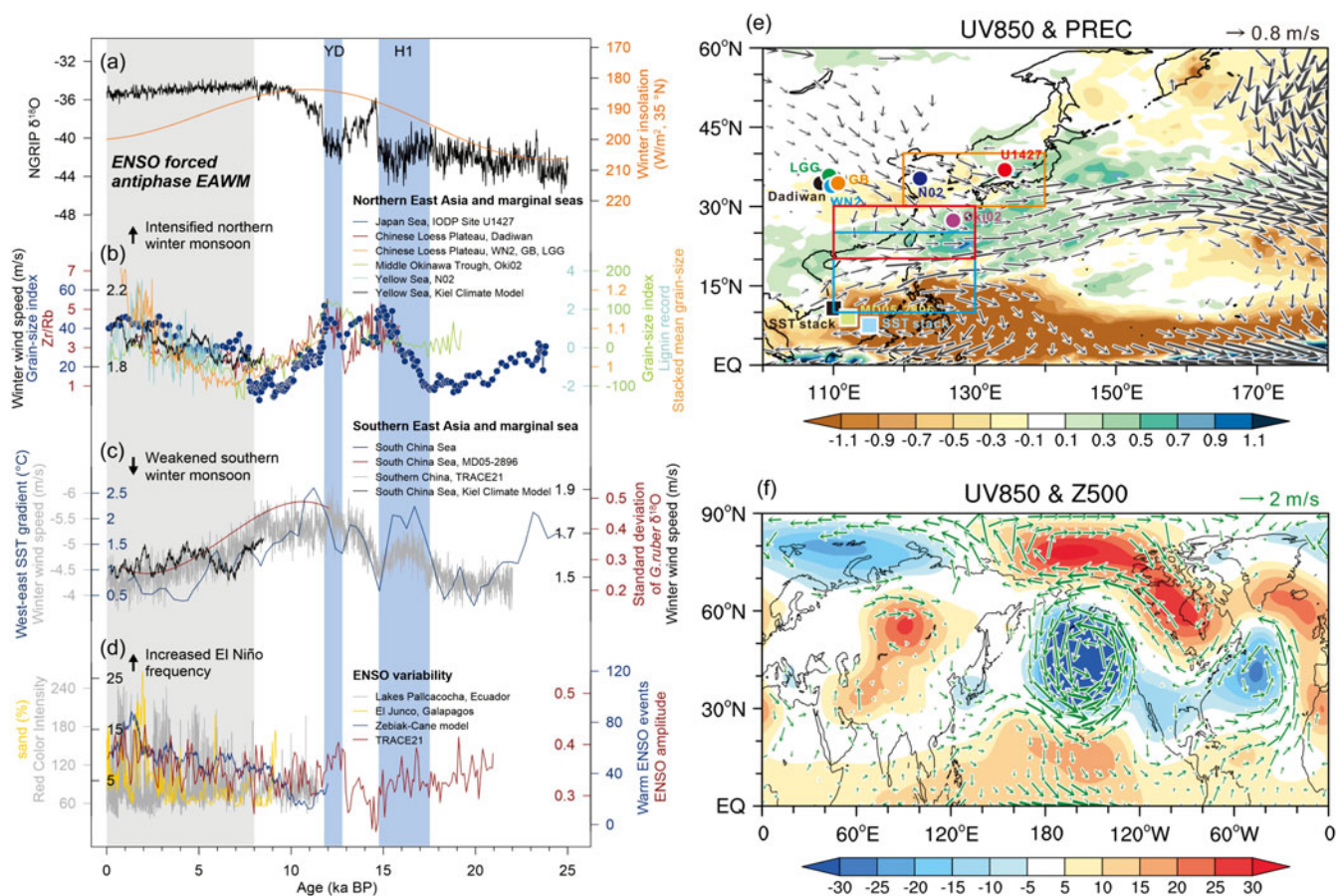
Figure 6. (Colour online) Comparison between EAWM with its potential forcing mechanisms. (a) NGRIP \delta^{18}\text{O} record (Andersen et al. 2004) and winter insolation in 35°N (Laskar et al. 2004). (b) EAWM reconstructions and simulation in the northern East Asia and its marginal seas. (c) EAWM reconstructions and simulation in the southern East Asia and marginal sea. (d) ENSO reconstructions and simulation (Clement et al. 2000; Conroy et al. 2008; Liu et al. 2014b; Moy et al. 2002). (e) Regression coefficients of the 850-hPa wind (vectors in m/s) and rainfall anomalies (shadings in mm/day) with respect to the December, January and February (DJF) mean Niño-3.4 index for the midwinter (Geng et al. 2023). The EAWM records in the northern and southern regions are shown with dots and squares, respectively. Orange, red and blue boxes show the regions of model simulation. (f) Regression coefficients of the 850-hPa wind (vectors in m/s) and 500-hPa geopotential height anomalies (shadings in m) with respect to the DJF mean Niño-3.4 index for the midwinter (Geng et al. 2023).
