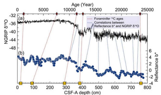
Figure 2. (Colour online) Age model of the top 7.75 m of the Hole A sediments at IODP Site U1427. The layers and their corresponding AMS 14 C dates are shown with yellow squares and red diamonds with black error bars, respectively, connected by red dotted lines. The blue dotted lines show the correlations between (a) NGRIP \delta^{18}\text{O} and (b) sediment reflectance b^* .
