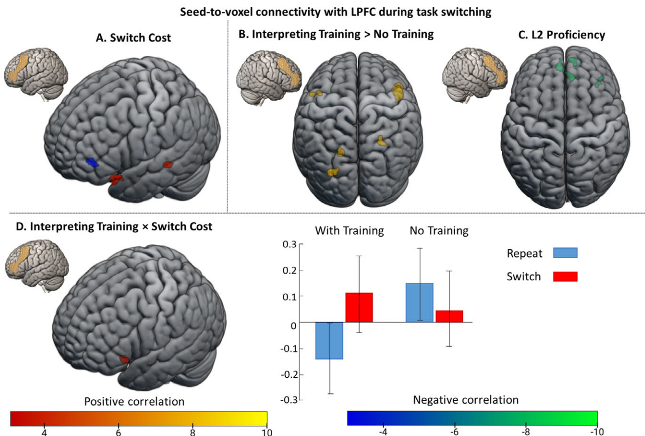
Figure 4. Seed-to-voxel task-based functional connectivity, using bilateral LPFC as seeds, is displayed in the small brown brains on the left corner. (A) Switch cost, red/yellow represents stronger connectivity in Switch than Repeat, while blue/green represents stronger connectivity in Repeat than Switch. (B) Across Switch and Repeat conditions, stronger connectivity in individuals with interpreting training than no training. (C) Across Switch and Repeat conditions, higher L2 proficiency is associated with weaker connectivity. (D) Regions that showed significant interaction with interpreting training and switch cost. Red/yellow suggests a positive correlation, whereas blue/green suggests a negative correlation. The color bar ranges from Z = 3.1 to Z = 10 .
