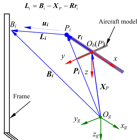
Figure 2. Illustration of the kinematic relationship in WDPR-8.
