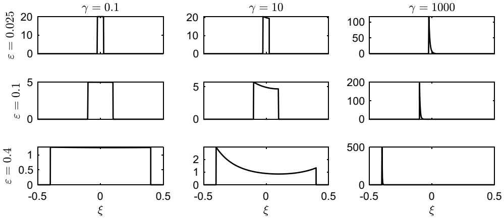
Figure 1. Plots of the Lebesgue density of \pi_1^{\gamma, \varepsilon}(\cdot | \theta_0) for energy \Phi(y_1 + \xi, z_1 | \theta_0) = (\xi - 0.1)^2/2 , choosing parameters \varepsilon \in \{0.025, 0.1, 0.4\} and \gamma \in \{0.1, 10, 1000\} .
