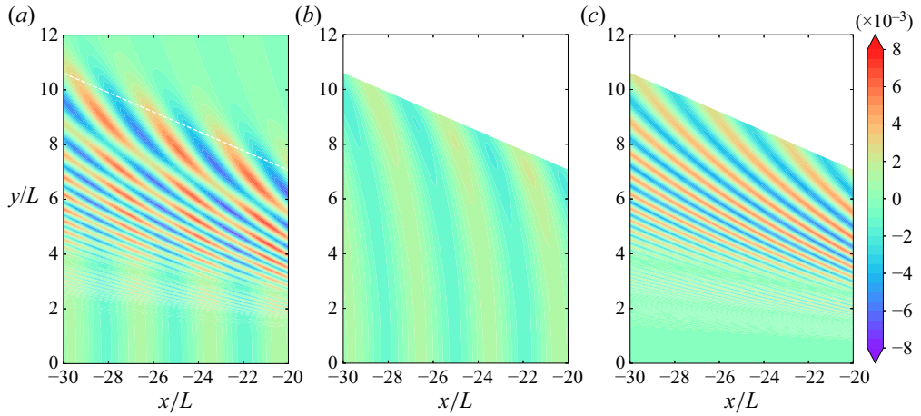
Figure 12. Same as figure 10, but F = 0.7 .
