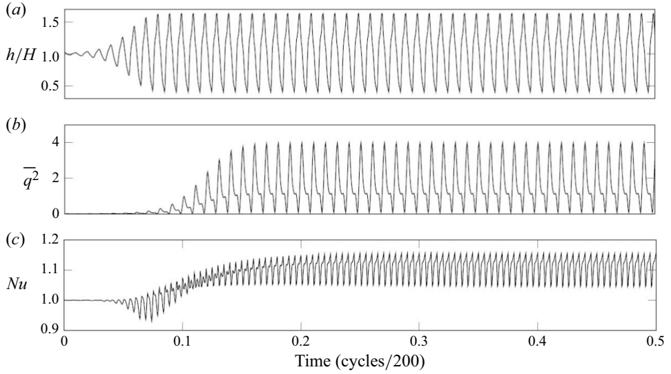
Figure 6. Simulated dynamics of a 10 cSt silicone oil ( Pr = 83.3 , \delta = 0.08 ) system subject to microgravity ( g = 0 \text{ m s}^{-2} ) in contact with a passive upper layer that is oscillated at an amplitude beyond the critical threshold ( \Omega = 1.3\Omega_c ) and beyond the natural subharmonic frequency ( f = 1.05f_{sub} ) such that the excited mode is k = 2\pi . The dynamics is expressed using (a) the anti-node of the interface h(x/W = 0.5, t) , (b) the x -integrated flow rate \overline{q^2} , and (c) Nu .
