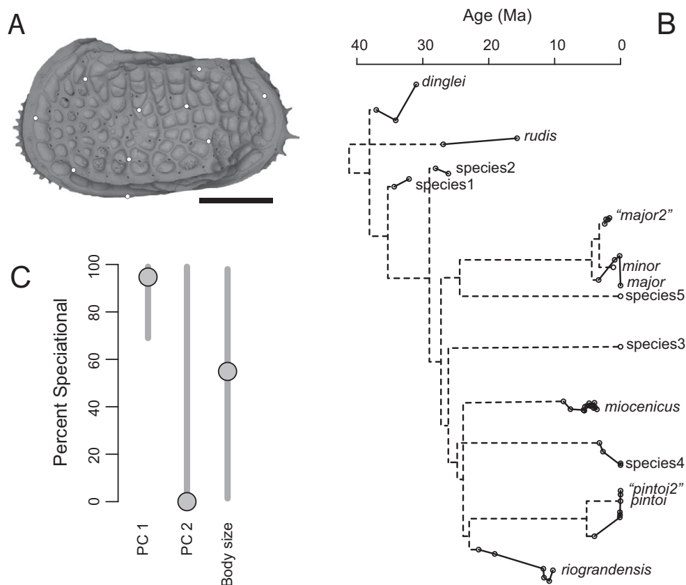
Figure 2. A, Representative of the ostracod genus Poseidonamicus with 10 landmarks used in morphological analysis; scale bar is 250 microns. B, Inferred phylogeny of the genus, with sampled anagenetic portions of the clade in solid lines. Population means are plotted vertically according to their mean scores on PC 1 and horizontally by their geological ages. C, Plot showing maximum-likelihood estimates (circles) and confidence intervals (vertical bars) for the proportion of evolutionary change in species attributable to speciation pulses. PC 1 and PC 2 accounted for 25% and 17% of the variation in the morphometric dataset, respectively. Body size was measured as log-transformed valve length.
