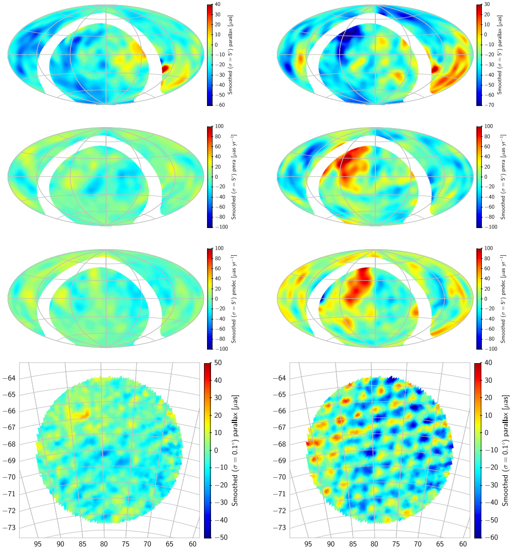
Figure 1. Figures 13 and 14 of Lindegren et al. (2021) . The three top panels show the all sky smoothed maps of quasars parallaxes and proper motions, while the low panels show the smoothed maps of parallaxes in the Large Magellanic Cloud area. Left panels are for EDR3/DR3 and right panels for DR2.
