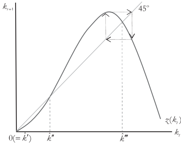
FIGURE 3. \nu = 0 and z'(\hat{k}''') < -1 : an example with a period-2 cycle.
