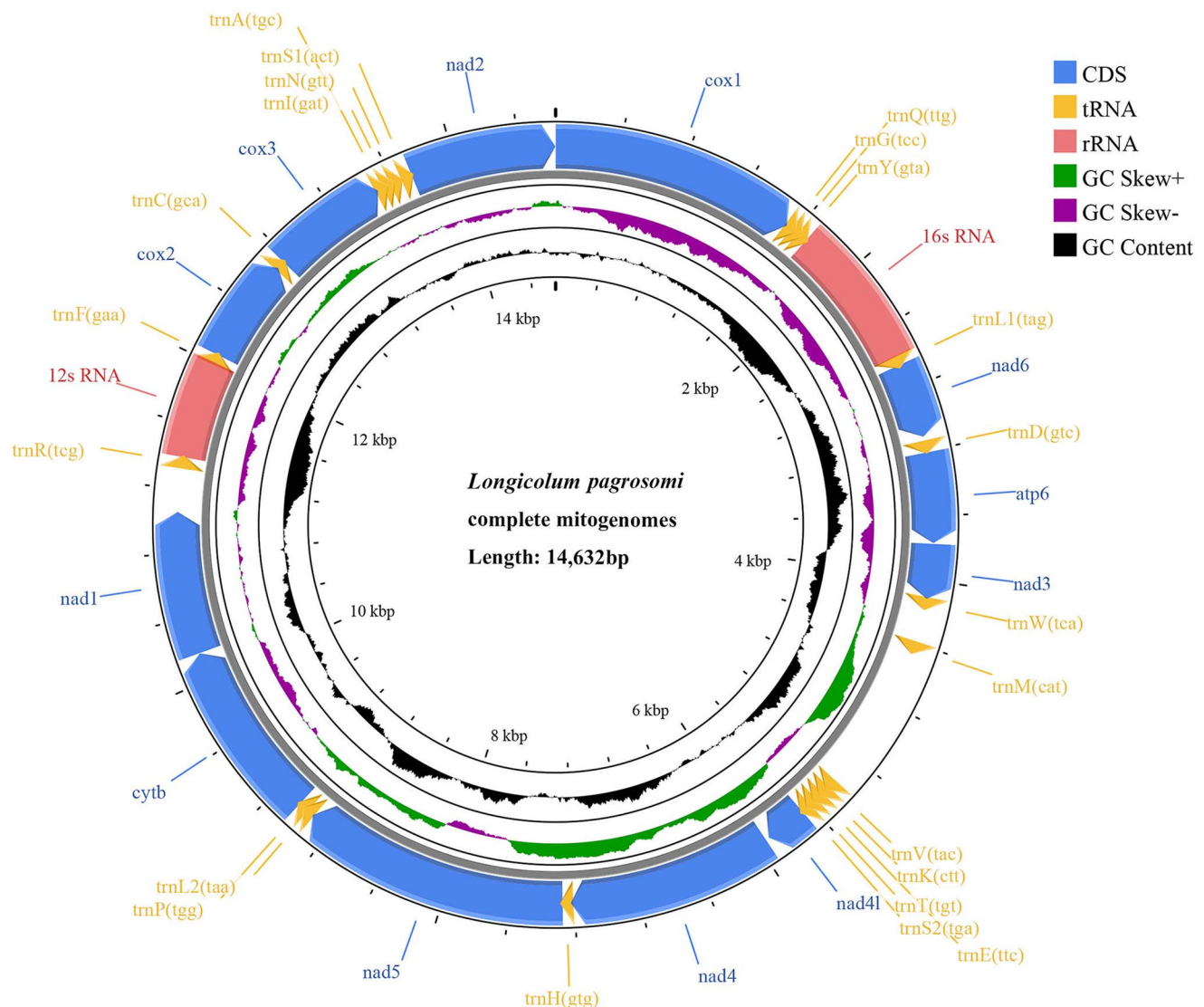
Figure 1. Map of the complete mitogenomes of Longicollum pagrosomi . 12 protein-coding genes (12) are shown in blue, rRNAs (2) in pink, and tRNAs (22) in yellow.
