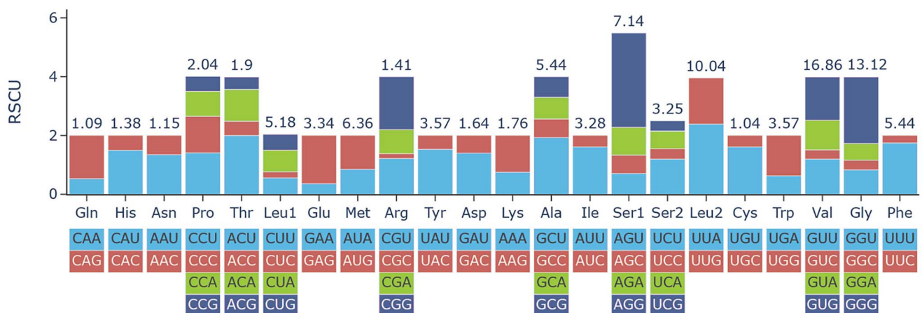
Figure 2. Relative synonymous codon usage (RSCU) of the complete mitogenomes of L. pagrosomi . Codon families are labelled on the x-axis. Values on the top of the bars refer to amino acid usage.
