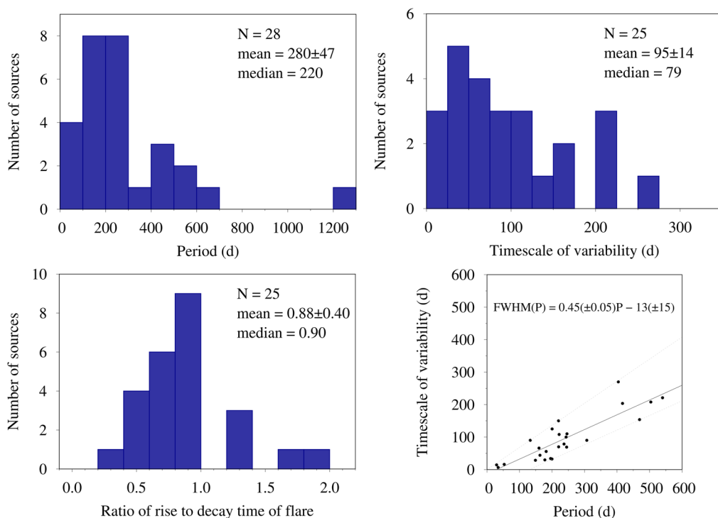
Figure 1. Distributions of selected variability parameters of known periodic sources from Table A3 in Olech et al. 2019 updated with new objects reported by Olech et al. (2022) and Tanabe et al. (2023).
