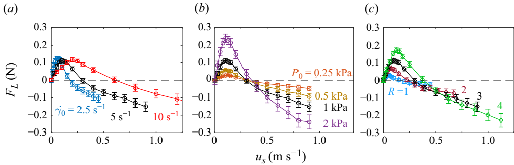
Figure 4. Lift-force F_L vs. slip velocity u_s for a non-rotating intruder with varying (a) \dot{\gamma}_0 with R = 3 , P_0 = 1000 Pa, (b) P_0 with R = 3 , \dot{\gamma}_0 = 5 \text{ s}^{-1} and (c) R with P_0 = 1000 Pa, \dot{\gamma}_0 = 5 \text{ s}^{-1} . Note that two data points at large u_s > 1.25 \text{ s}^{-1} for \dot{\gamma}_0 = 10 \text{ s}^{-1} in (a) are not shown to keep the horizontal axes consistent in all three panels.
