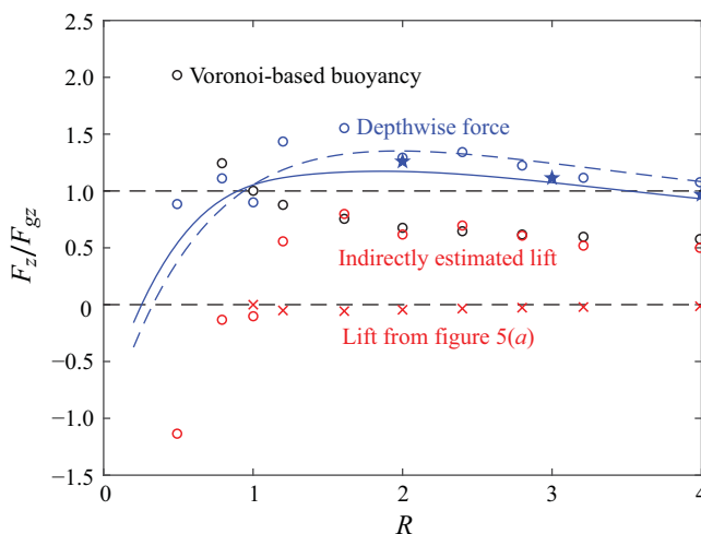
Figure 18. Comparison of segregation force F_z normalized by intruder weight in the cross-flow direction, F_{gz} , vs. the size ratio, R . Data from van der Vaart et al. (2018) ( \circ ) show the total cross-flow force (blue), the Voronoi-based buoyancy force (black) and the indirectly estimated lift force due to slip velocity (red) and are compared with the lift force calculated using figure 5(a) and the cross-flow total force ( \star ) in Yennemadi & Khakhar (2023). The blue solid curve shows the predicted total segregation force and the blue dashed curve shows the buoyancy due to the pressure gradient based on Jing et al. (2021).
