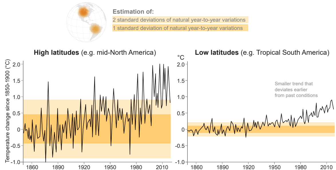
FAQ 1.2, Figure 1 | Observed variations in regional temperatures since 1850 (data from Berkeley Earth). Regions in high latitudes, such as mid-North America (40°N–64°N, 140°W–60°W, left ), have warmed by a larger amount than regions at lower latitudes, such as tropical South America (10°S–10°N, 84°W–16°W, right ), but the natural variations are also much larger at high latitudes (darker and lighter shading represents 1 and 2 standard deviations, respectively, of natural year-to-year variations). The signal of observed temperature change emerged earlier in tropical South America than mid-North America even though the changes were of a smaller magnitude. (Note that those regions were chosen because of the longer length of their observational record; see Figure 1.14 for more regions).
