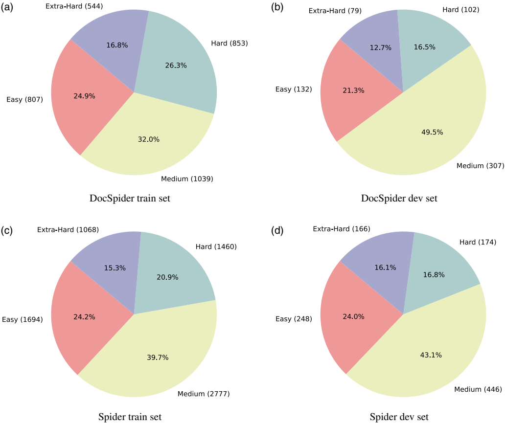
Figure 5. Difficulty level distribution of the queries in the data splits.
