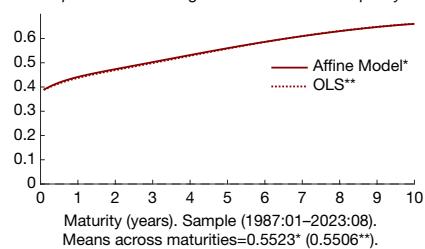
Graph F. Yield Loadings: Nominal USTs: 5. Liquidity*
