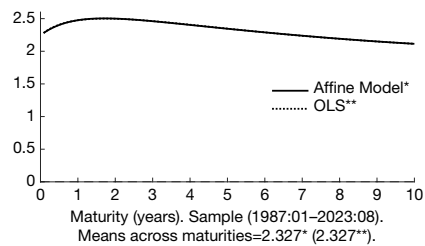
Graph D. Yield Loadings: Nominal USTs: 3. Curvature*
