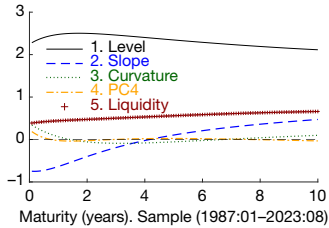
Graph A. Affine Model Yield Loadings: Nominal USTs
