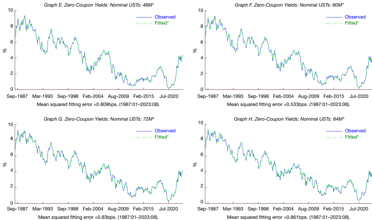
FIGURE 5 (continued) Model Implied Yields: Time Series
