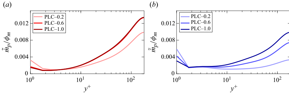
Figure 11. Variation of normalised particle average mass flow rate ( \tilde{m}_p = \bar{m}_p / m_0 ) per unit mass loading along the channel height for different PLC flows with (a) St^+ = 6 and (b) St^+ = 30 . Darker curves correspond to higher particle mass loadings varying from 0.2 to 1.0.
