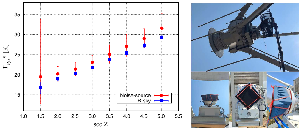
Figure 6. (Left) System noise temperature T_{\text{sys}}^* (included atmosphere) versus \sec Z . T_{\text{sys}}^* measured with injecting the noise-source and R-sky methods are shown by circle and square symbols, respectively. (Right) scene in temporal installation of an absorber on top of the L-band horn (detached already).
