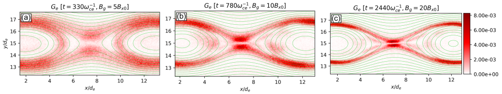
FIGURE 10. Electron agyrotropy G_e in all three cases. The three panels share the same colourbar, which is located on the far right-hand side of the figure.
