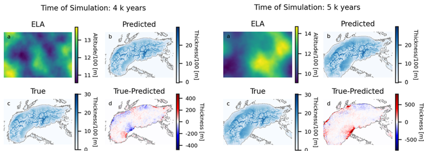
Figure 3. Emulator evaluation at two distinct run times (4 and 5 ka) to illustrate its predictive capabilities. (a) ELA field used as input for the IGM and the emulator. (b) Emulator-predicted GMT. (c) GMT from the IGM. (d) Difference between true and predicted GMT (blue: overestimation; red: underestimation). Overall, the emulator closely replicates the IGM outputs.
