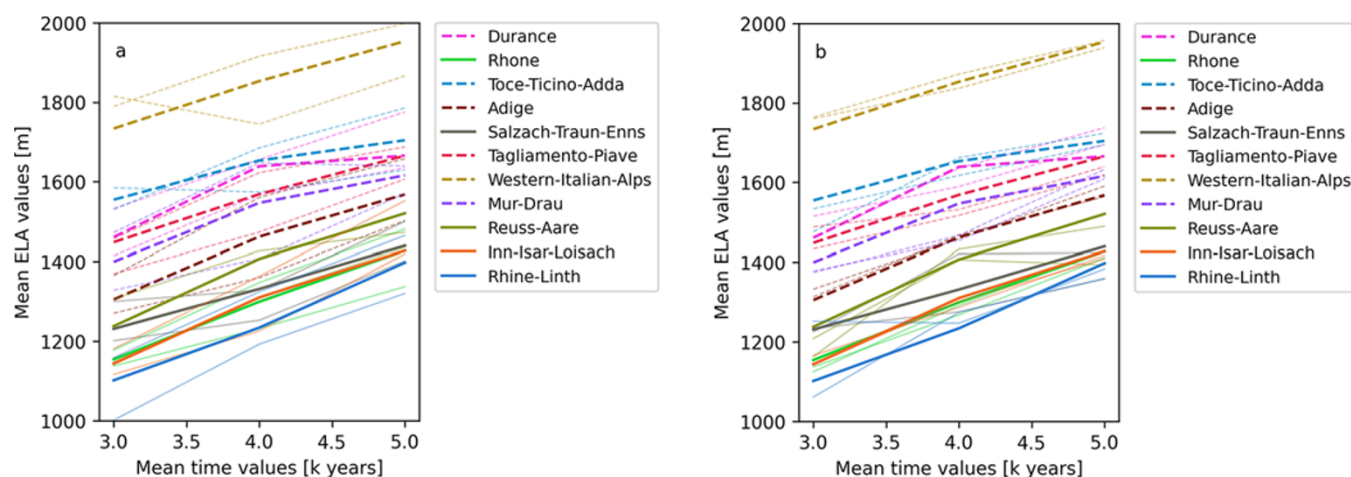
Figure 7. (a) Sensitivity of mean ELA values to variations in the mass balance gradient \beta_{abl} . (b) Sensitivity of mean ELA values to variations in the rate factor in Glen's flow law (4). Mean values from standard parameters are in bold colours, while halved and doubled parameters are shown with reduced opacity. Solid lines indicate northern regions; dashed lines represent southern regions.
