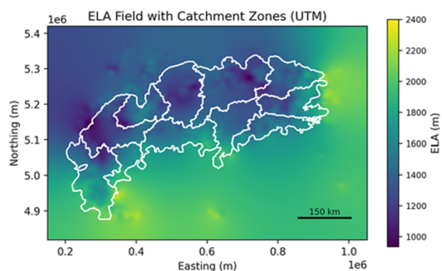
Figure 5. The ELA map obtained from the inversion scheme using the parameters: T = 4000 a, A = 78 \text{ MPa}^{-3} \text{ a}^{-1} , \beta = 0.008 \text{ a}^{-1} , s = 2.1 \text{ km MPa}^{-3} \text{ a}^{-1} and \lambda = 0.1 . The ELA map is delineated by predefined catchments (Fig. 4). The map reveals a distinct gradient, with ELA values increasing from northwest to southeast.
