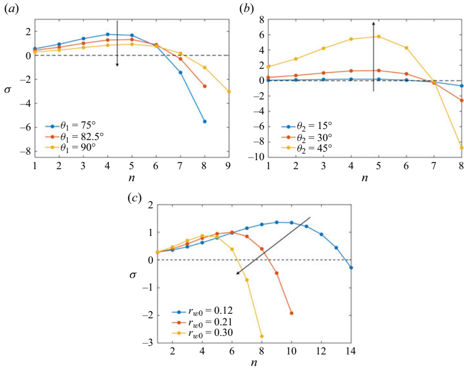
Figure 6. Growth rate curves for: (a) r_{w0} = 0.26 , \theta_2 = 30^\circ and \theta_1 = 75^\circ, 82.5^\circ and 90^\circ ; (b) r_{w0} = 0.26 , \theta_1 = 82.5^\circ and \theta_2 = 15^\circ, 30^\circ and 45^\circ ; and (c) \theta_1 = 90^\circ , \theta_2 = 30^\circ and r_{w0} = 0.12, 0.21 and 0.30 . The arrows show the direction of increasing \theta_1 in (a), \theta_2 in (b) and r_{w0} in (c).
