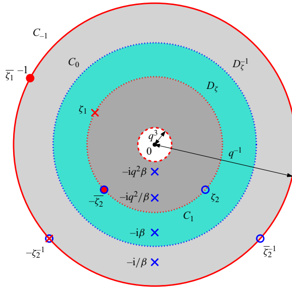
Figure 3. The annuli appearing in the analysis. D_\zeta^{-1} (light grey) is the reflection of the pre-image domain D_\zeta (turquoise) of figure 2 in the unit circle C_0 (dotted blue). The union of \overline{D_\zeta} and D_\zeta^{-1} forms the fundamental region F of (3.4) for the group \Theta . The union of \overline{F} and the reflection of F in the circle C_1 (dotted red) forms the fundamental region \tilde{F} of (3.10) for the group \tilde{\Theta} . The complex velocity W'(\zeta) has simple poles (blue crosses) at \zeta = -i\beta, -i/\beta, -iq^2\beta and -iq^2/\beta , and simple zeros (blue circles) at \zeta = \zeta_2, -\zeta_2, 1/\zeta_2 and -1/\zeta_2 . ( -\zeta_2 = \zeta_3 – see (3.25).) The mapped complex velocity \Omega(\zeta) has simple poles (red crosses) at \zeta = \zeta_1 and -1/\zeta_2 (coinciding with a zero of W'(\zeta) ), and simple zeros (red discs) at \zeta = 1/\zeta_1 and -\zeta_2 (also coinciding with a zero of W'(\zeta) ).
