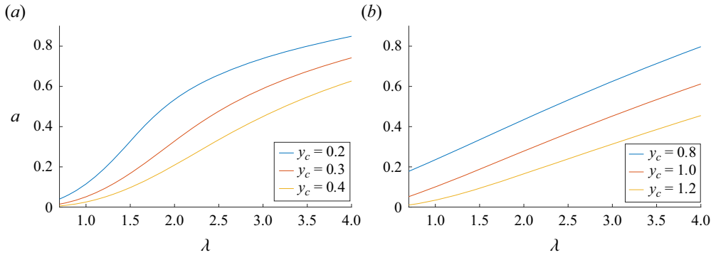
Figure 6. The surface disturbance amplitude, a , i.e. the vertical height between a peak and a trough, as a function of \lambda for various leading-edge submergences y_c and angles of attack: (a) -\alpha = \pi/4 ; (b) -\alpha = -\pi/3 .
