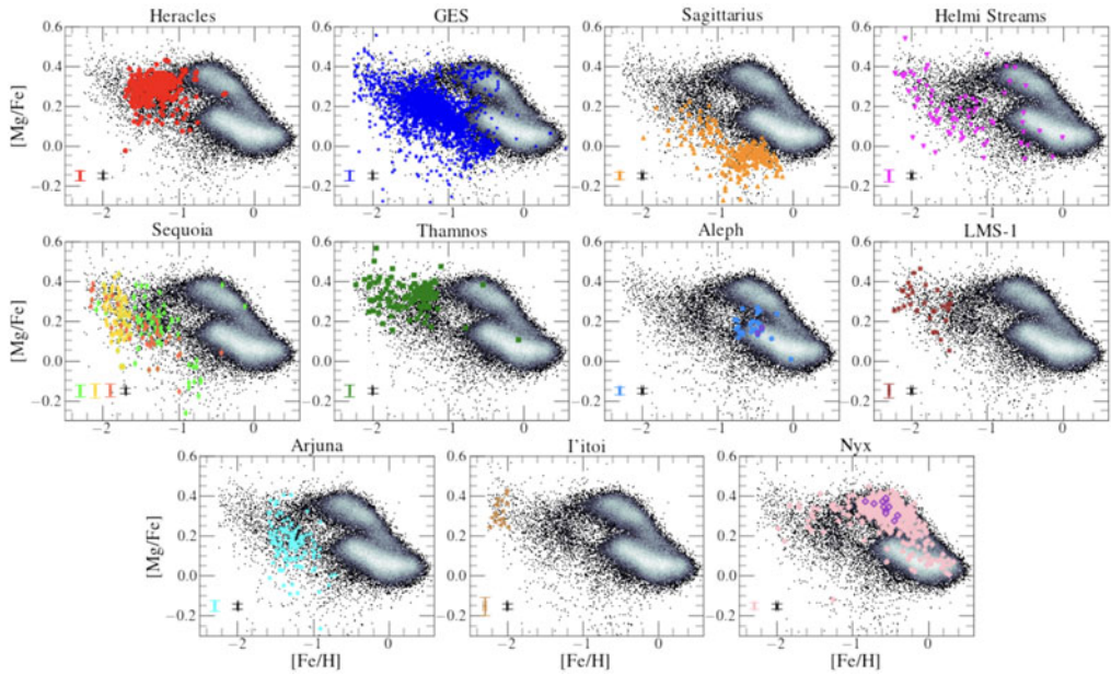
Figure 1. The resulting parent sample and identified structures in the Mg-Fe plane. The mean uncertainties in the abundance measurements for halo substructures (colour) and the parent sample (black) are shown in the bottom left corner. For the Aleph and Nyx substructures, we also highlight with purple edges stars from our APOGEE DR17 data that are also contained in the Aleph and Nyx samples from the Naidu et al. 2020 and Necib et al. 2020 samples, respectively.
