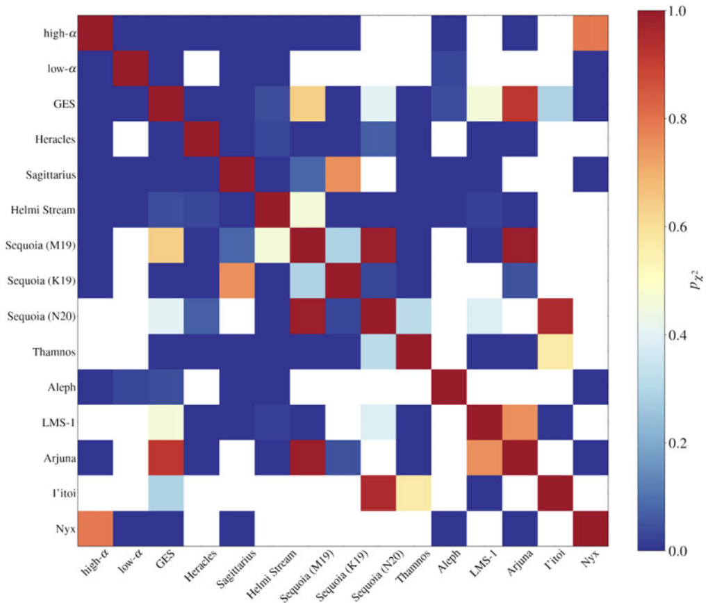
Figure 2. Confusion matrix of the probability values obtained when comparing the chemical compositions of all the halo substructures with each other and with a high-/low- \alpha discs. Here, each substructure is compared with its counterpart using a [\text{Fe}/\text{H}] value that is well covered by the data, where red(blue) signifies a high(low) probability of two systems being statistically similar given their chemical compositions. Comparisons with blank values are due to the two substructures being compared not having any overlap in [\text{Fe}/\text{H}] .
