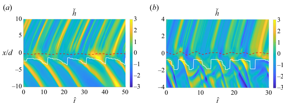
Figure 13. Spatiotemporal contours of the normalized film thickness \tilde{h} for cases (a) 1 and (b) 3, complemented with the temporal evolution of the impingement point x_p (dashed red line) and the wiping point x^* (continuous white line), both defined in the text. (a) Case 1 (DG); (b) case 3 (W).
