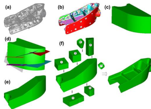
Figure 2. Complete model reconstruction ( Wang et al., 2012 ): (a) point cloud (b) segmentation result (c) outer block extrusion (d) detected planes (e) trimming with planes (f) detecting all other features; resemble the model using boolean operations
