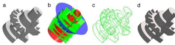
Figure 3. Model reconstruction (Bénière et al., 2013): (a) 3D mesh (b) extracted geometric primitives (c) reconstructed wires (boundaries) (d) final BREP model
