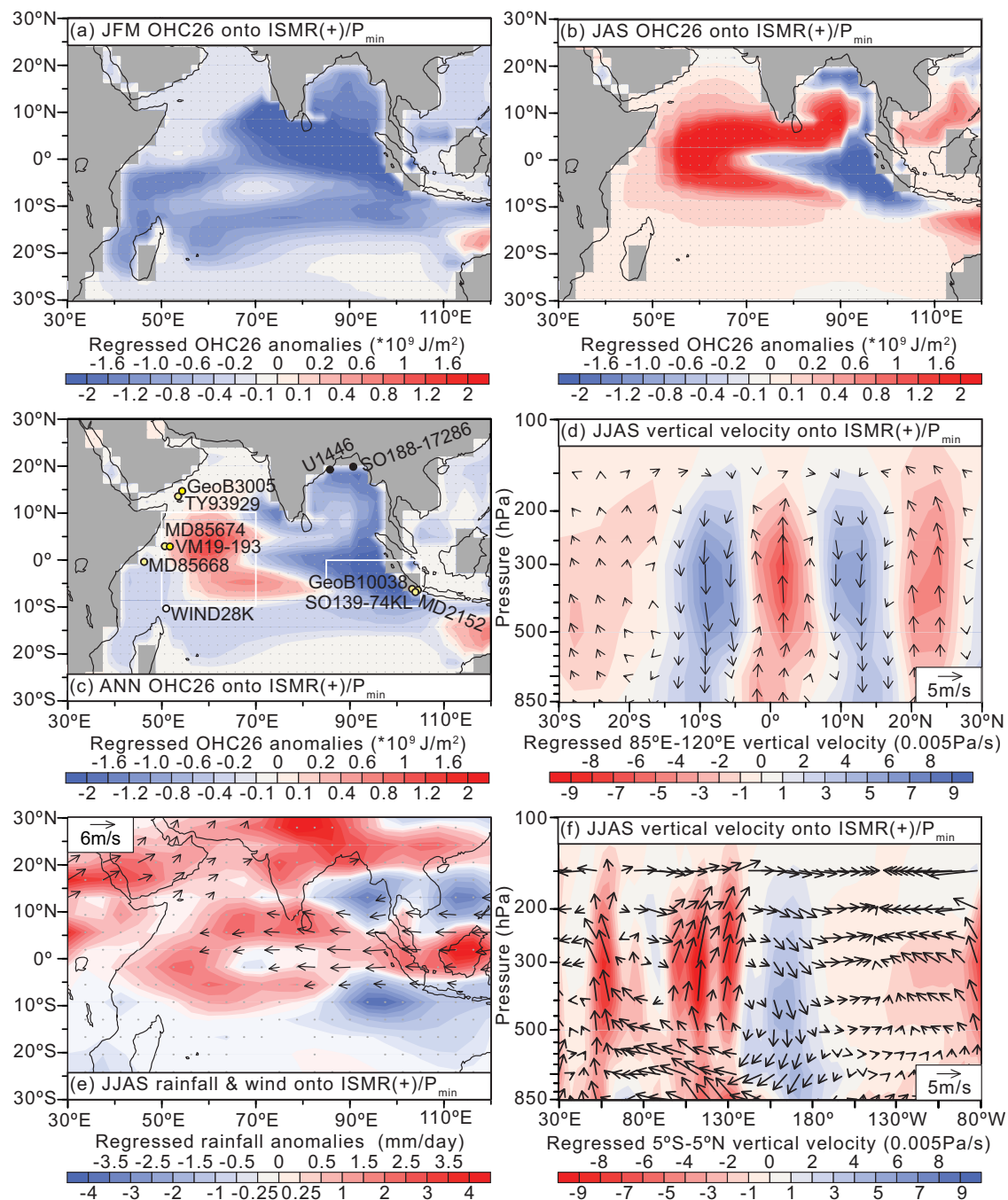
Figure 5. (Colour online) Regression coefficients against the normalized time series of ISMR_{CESM} from experiment CESM_{ghg} . (a)–(c) are JFM, JAS and annual mean OHC. (d) JJAS vertical p velocity (shaded) and meridional vertical circulation (vectors; meridional wind v and vertical p velocity) along the longitudes 85^{\circ} E– 120^{\circ} E, (e) JJAS rainfall (shaded) and 850 hPa horizontal winds (vectors, small winds (magnitude < 2 m/s) are not shown). (f) JJAS vertical p velocity (shaded) and zonal-vertical circulation (vectors; zonal wind u and vertical p velocity) along the latitudes 5^{\circ} S– 5^{\circ} N. White rectangular in (c) show the WIO and EIO regions for calculating DMI in simulations (Wang et al. 2015). Yellow, white, and black filled dots in (c) show site locations of paleo-proxies ( U^{K}_{37} -SST, Mg/Ca-SST and \delta^{18}O_{sw} ). Character “ISMR(+)/ P_{min} ” means that these anomalies are regressed onto the ISMR maximum (also the minimum of precession parameter).
