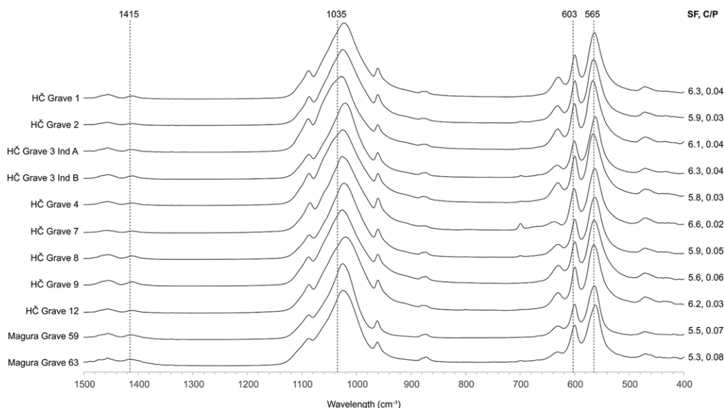
Figure 5. Results of FTIR measurements on cremated bones from Hajdučka Česma and Magura (L. Webster).
