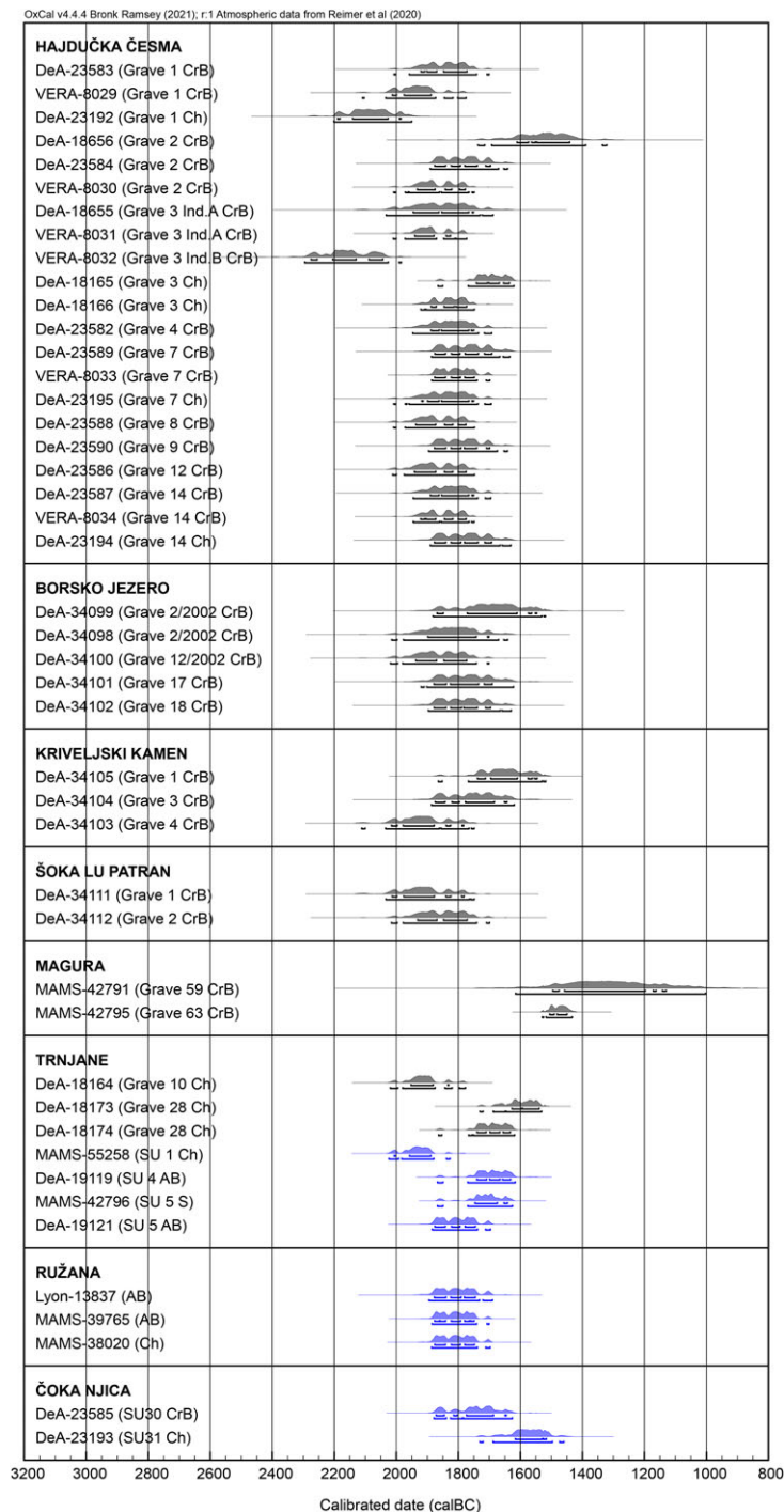
Figure 6. Independently calibrated ^{14}\text{C} dates from urn cemeteries and settlements of copper-producing societies in eastern Serbia. The type of material dated is indicated in brackets: CrB = cremated bone, Ch = charcoal, AB = animal bone, S = seed. Highest probability density (hpd) ranges for 68.3% and 95.4% are marked with bars below each result. Blue indicates dates from settlement rather than cemetery contexts. Two outliers, DeA-18167 and De-18168 (10th century AD) are not shown.
