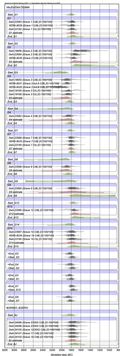
Figure 7. Bayesian analysis for Hajdučka Česma and Borsko Jezero. Individual probability distributions before and after modeling are shown in light and dark grey respectively. Calculated transition boundaries are colored green and phase estimates red. Highest posterior density (hpd) ranges after modeling (68.3% and 95.4%) are marked with bars below each result. The model uses OxCal's outlier analysis to account for possible outliers and offsets. This preferred version of the model uses a normal distribution with an offset ( -30 \pm 15 years) to allow for inbuilt and minor "old age" effects in the cremated bone.
