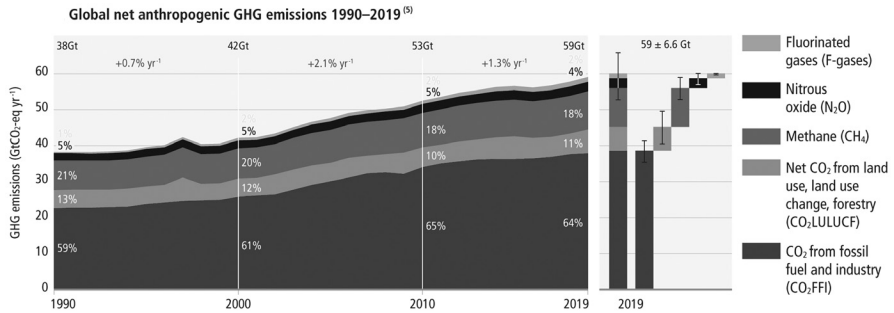
FIGURE 2.2 Global net anthropogenic GHG emissions (GtCO 2 -eq yr -1 ) 1990–2019. Global net anthropogenic GHG emissions include CO 2 from fossil fuel combustion and industrial processes (CO 2 -FFI); net CO 2 from land use, land-use change, and forestry (CO 2 -LULUCF); methane (CH 4 ); nitrous oxide (N 2 O); and fluorinated gases (HFCs, PFCs, SF 6 , NF 3 ). At the right side of the panel, associated uncertainties for each of the components for 2019 are shown. 22
