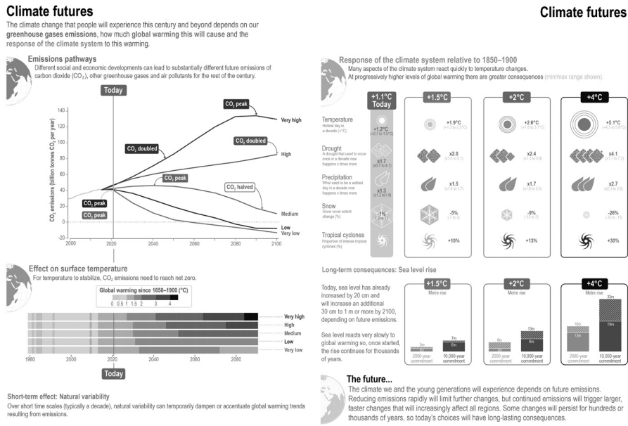
FIGURE 2.7 Linking carbon dioxide emissions, global warming, and effects on the climate systems. Panel (a): Top – Annual emissions of carbon dioxide for the five core Shared Socioeconomic Pathway (SSP) scenarios (very low: SSP1–1.9, low: SSP1–2.6, medium: SSP2–4.5, high: SSP3–7.0, very high SSP5–8.5). These scenarios are illustrative, meaning that they are not intended to be predictions of what will happen in the future; instead they serve an informative purpose to see how the Earth will respond to different situations. Bottom – Projected warming for each of these emissions scenarios. This figure is sourced from the Technical Summary Infographic. Panel (b): Top – How temperature extremes, droughts, heavy rainfall (precipitation) events, snow cover, and tropical cyclones change at different levels of global warming compared with the late nineteenth century (1850–1900). Today, here is the average over 2011–2020. Bottom – Long term (2,000 and 10,000 years) committed sea level rise for global warming of 1.5°C, 2°C, and 4°C). 52
