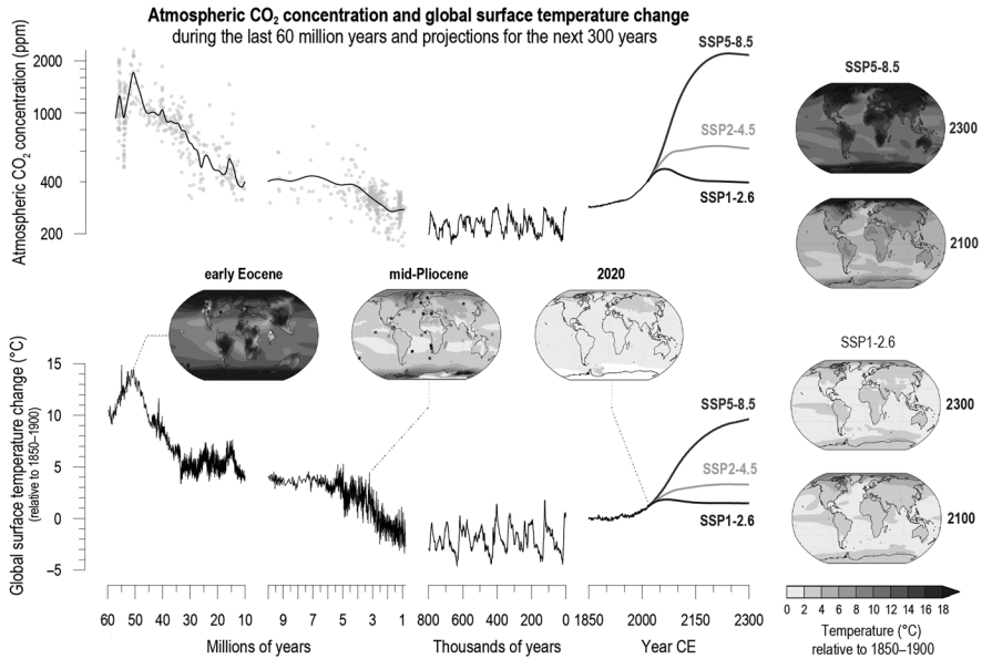
FIGURE 2.1 Historical records of global carbon dioxide concentration levels (parts per million, ppm) and temperature ( ^{\circ}\text{C} ) over the past 60 million years. For context, humans developed around 250,000 years ago, and agriculture only developed 10,000 years ago with a more stable and warmer climate. 13
