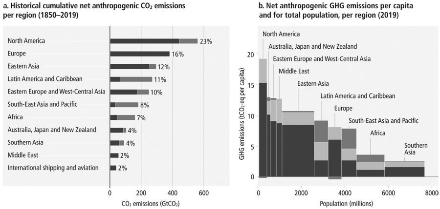
FIGURE 2.3 Regional differentiations of greenhouse gas emissions. Panel (a): Cumulative regional carbon dioxide emissions from 1850 to 2019. Panel (b): Regional GHG emissions in tonnes CO 2 -eq per capita by region in 2019. Note that emissions from international aviation and shipping are not included. Key: Black = CO 2 from fossil fuel combustion and industrial processes (CO 2 -FFI); Dark grey = net CO 2 from land use, land-use change, and forestry (CO 2 -LULUCF); Light grey = Other GHG emissions. 26
