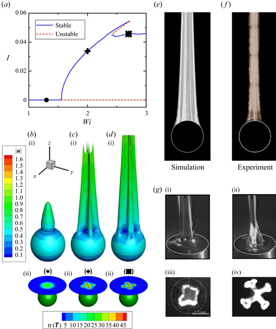
Figure 6. (a) Asymmetry parameter versus Weissenberg number for \beta = 0.1 and B_R = 0.25 . The solution branches are obtained by direct steady-state simulations assuming symmetry across the x = 0 and y = 0 planes. The stability of the branches is determined by transient simulations of the whole geometry for Wi = 2 and 3 . (b i, c i, d i) Iso-surfaces of the dimensionless stress tensor trace ( \text{tr}(\mathbf{T}) = 20 ) with superimposed dimensionless velocity magnitude ( |\mathbf{u}| ) contours for (b) Wi = 1.3 , (c) Wi = 2 , (d) Wi = 2.7 on the stable solution branch ( \beta = 0.1 , B_R = 0.25 ). (b ii, c ii, d ii) Contours of the dimensionless stress tensor trace on the plane z = 1.4 for (b) Wi = 1.3 , (c) Wi = 2 , (d) Wi = 2.7 on the stable solution branch ( \beta = 0.1 , B_R = 0.25 ). (e, f) Visual comparison between iso-surfaces of the dimensionless stress tensor trace ( \text{tr}(\mathbf{T}) = 50 ) obtained from simulations ( Wi = 3.5 , \beta = 0.1 , B_R = 0.25 ) and experimentally measured flow-induced birefringence for a steel ball falling in a polystyrene solution ( Wi \approx 3.5 ) (Howard 1998). (g) Elongation of viscoelastic fluid filaments: (g i, ii) side views for increasing strain, (g iii, iv) bottom views through a glass endplate for increasing strain. Reproduced with permission from Anna, Spiegelberg & McKinley (1997). Copyright 1997, AIP Publishing LLC.
