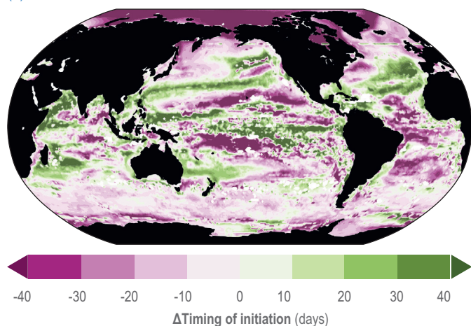
(c) SSP5-8.5
