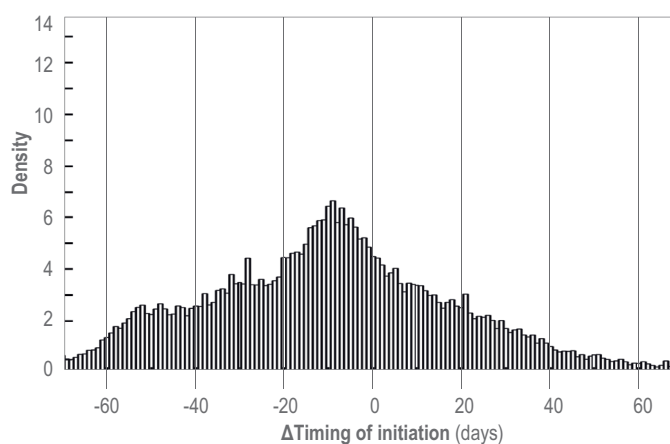
Figure 3.17 | Projected phytoplankton phenology. (a,c) Spatial patterns and (b,d) density distributions of projected change in phytoplankton phenology by 2100 under Shared Socioeconomic Pathway (SSP)1-2.6 and SSP5-8.5, respectively. Difference in the start of the phytoplankton growth period is calculated as 2090–2099 minus 1996–2013. Negative (positive) values indicate earlier (later) start of the phytoplankton growth period by 2100. The ensemble projections of global changes in phytoplankton phenology include, under SSP1-2.6 and SSP5-8.5, respectively, a total of five Coupled Model Intercomparison Project 6 Earth system models containing coupled ocean biogeochemical models that cover a wide range of complexity (Kwiatkowski et al., 2019). (The phenology calculations are based on Racault et al., 2017, using updated data.)
