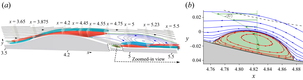
Figure 11. (a) Isosurfaces of \langle \omega_x \rangle = (-0.33, 0.33) along with the streamlines at the centre of grooves for reference; the grey Y - z planes denote location for colour maps in figure 10. (b) Zoomed-in view of streamlines around the secondary recirculation bubble (minibubble) within grooves at the location denoted by the dashed line box in panel (a).
