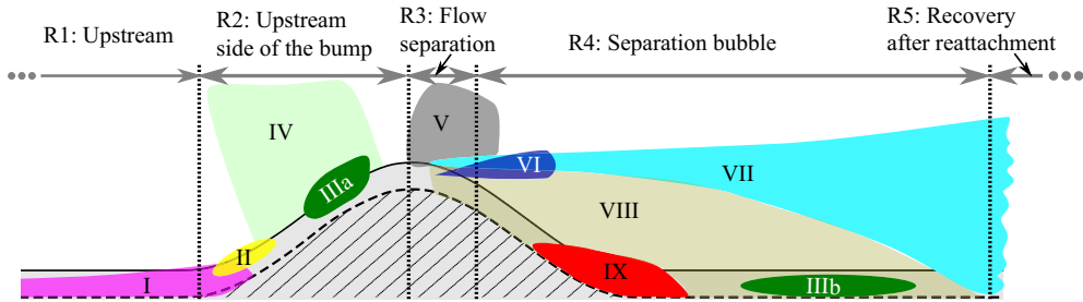
Figure 2. Schematic denoting the regions of interest and important flow features as a summary. I – upstream separation; II – incipient separation; IIIab – negative production; IV – favourable pressure gradient (FPG); V – adverse pressure gradient (APG); VI – spinning jets; VII – shear layer; VIII – separation bubble; IX – minibubble.
