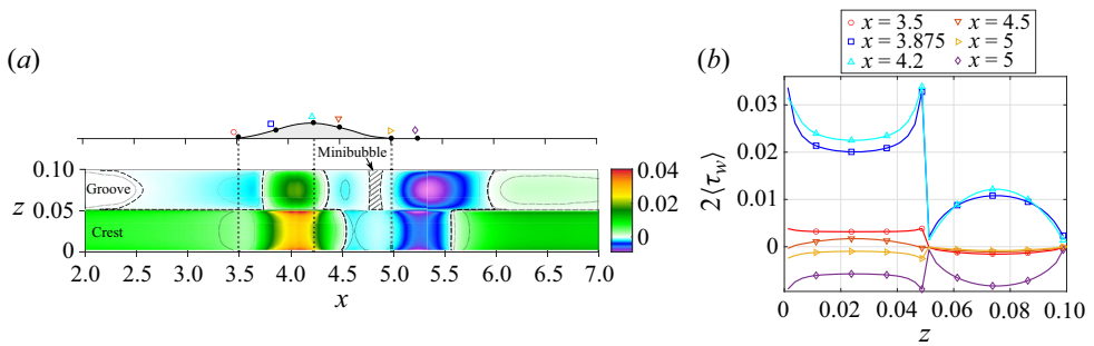
Figure 14. (a) Colour map of wall shear stress, 2\tau_{w,x} , for GW. The dashed line contour corresponds to \langle\tau_w\rangle = 0 . (b) Skin-friction profiles in the z -direction at different streamwise positions. The lines in panel (b) correspond to the x position denoted by the black dots over the bump in panel (a).
